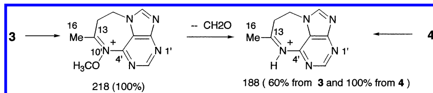
Figure 1. Major MS fragments of compounds 3 and 4 .
